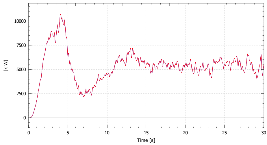
Torque (aero)
