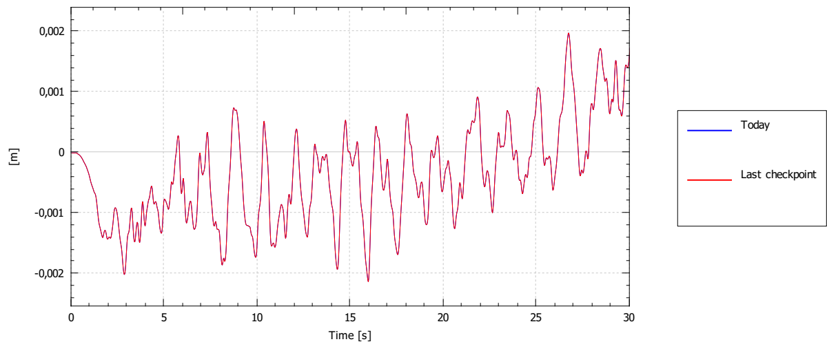
Displacement (w)
