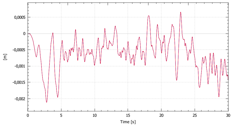
Displacement (w)
