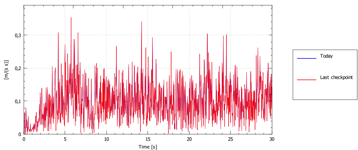
Acceleration, magnitude
